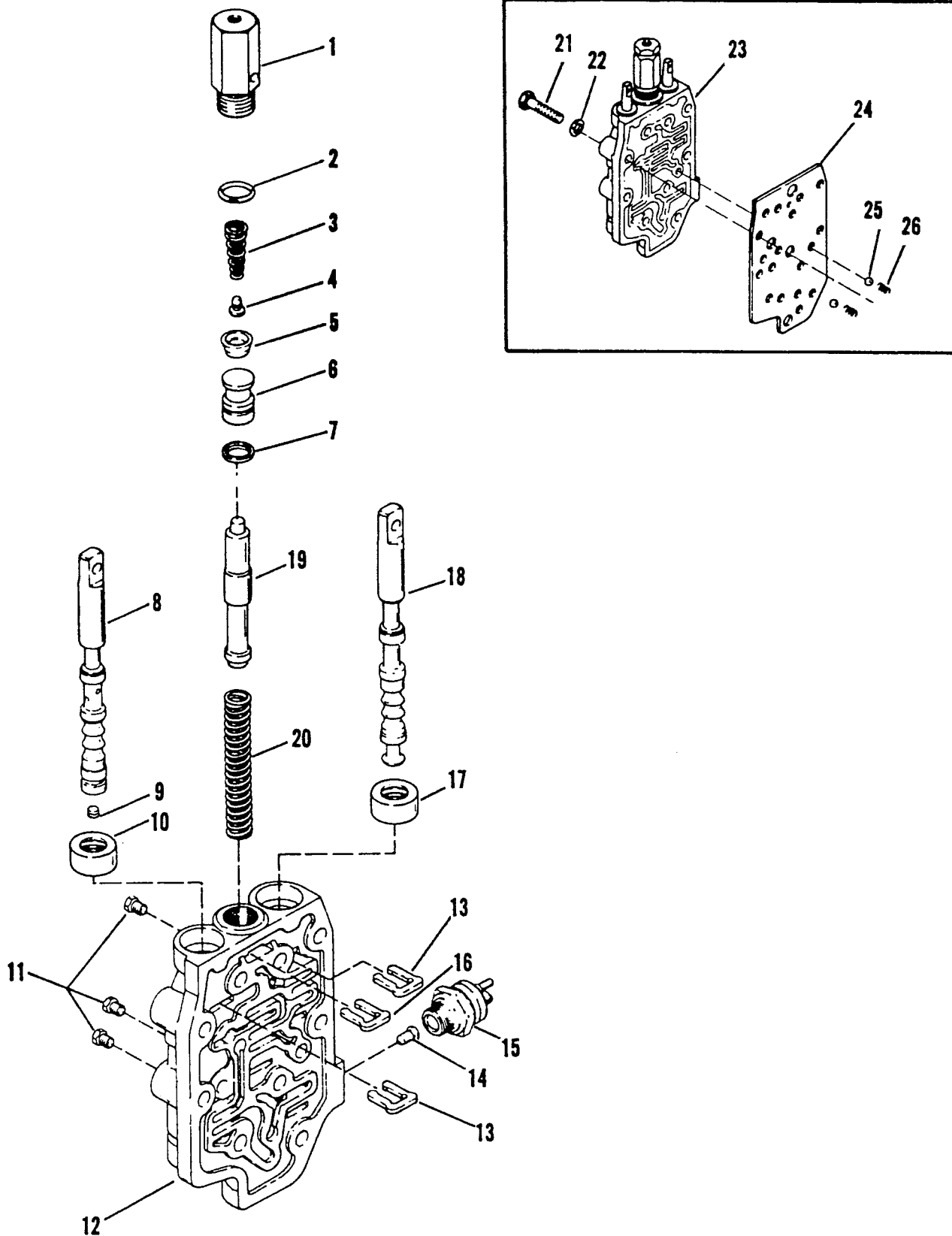
HYDRAULIC DECLUTCH
